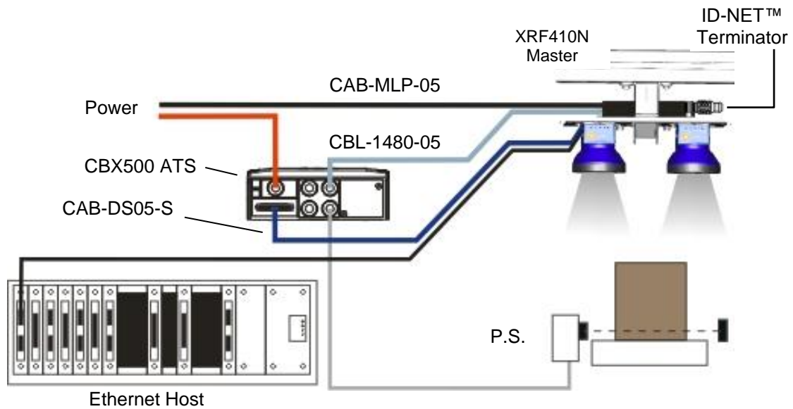
Figure 10 –Hxx Single Module Electrical Connections
