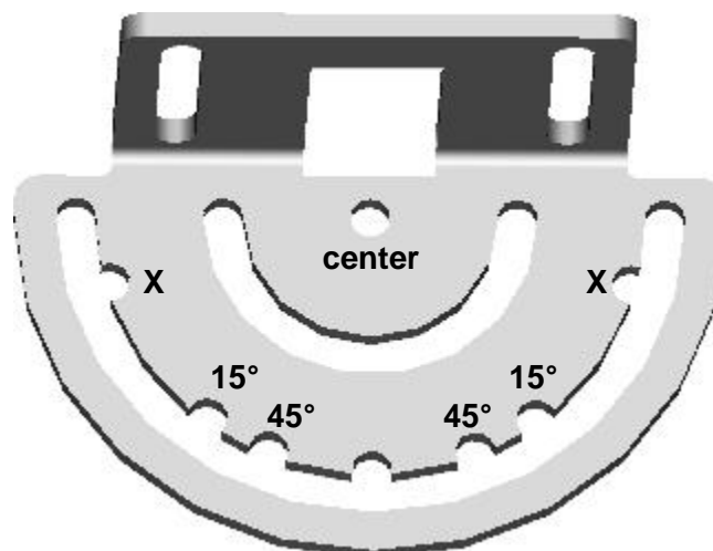
Figure 5 – Mirror Mounting Bracket
